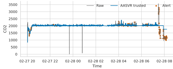
Figure 9: Representative CO 2 replay from the hydroponic deployment data. The trace shows the same trusted-state interface on an environmental-control stream, where transient raw readings should not directly authorize gas-release commands.
